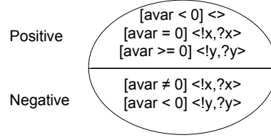
Figure 14: Semantics of guarded alt in Fig. 13
