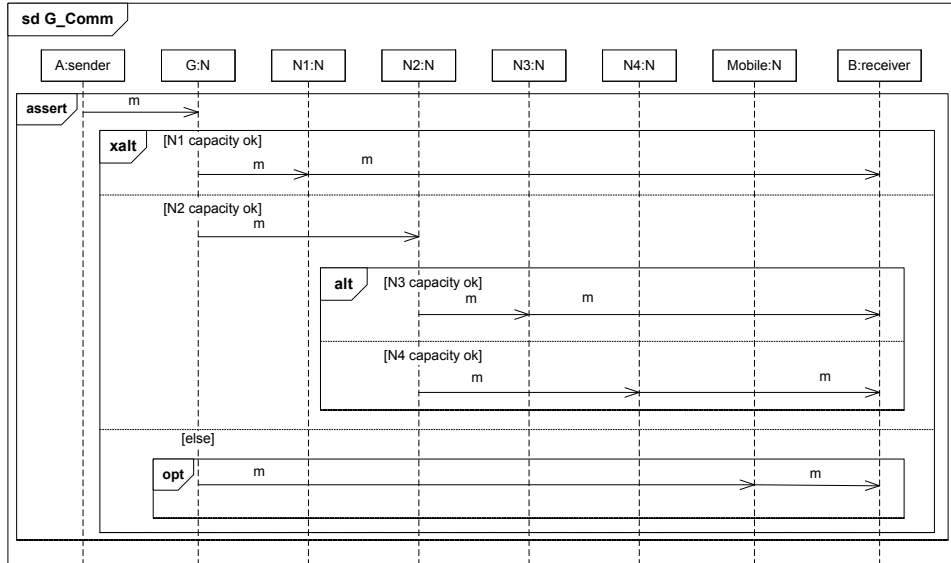
Figure 24: Introducing guards
