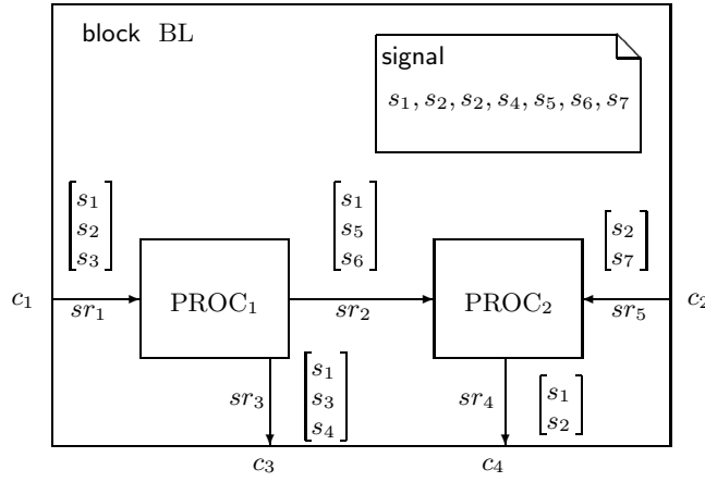
Figure 4: SDL Block Diagram
